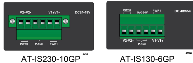
Figure 7. IS Series Power/Alarm Connectors
