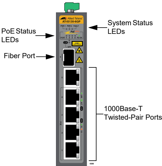
Figure 2. AT-IS130-6GP Switch Front Panel
