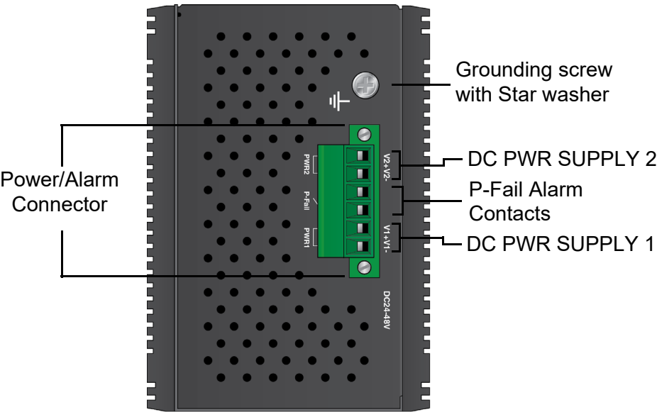
Figure 3. AT-IS230-10GP Switch Top Panel
