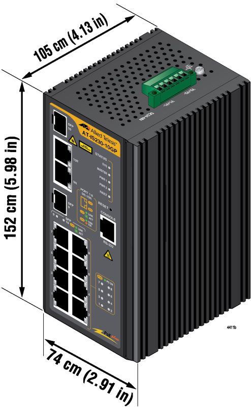
Figure 45. AT-IS230-10GP Dimensions
