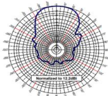
Elevation Pattern (Y, Z or H-Plane)
