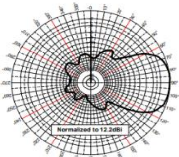
Azimuthal Pattern (X, Y or E-Plane)
