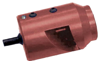
EZfit® Automated Cable Preparation Tool for AVA6-50 coaxial cable
