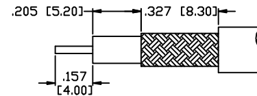
RECOMMENDED STRIPPING DIM'S
