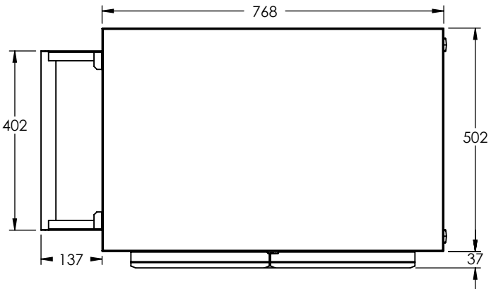
VISTA FRONTAL
