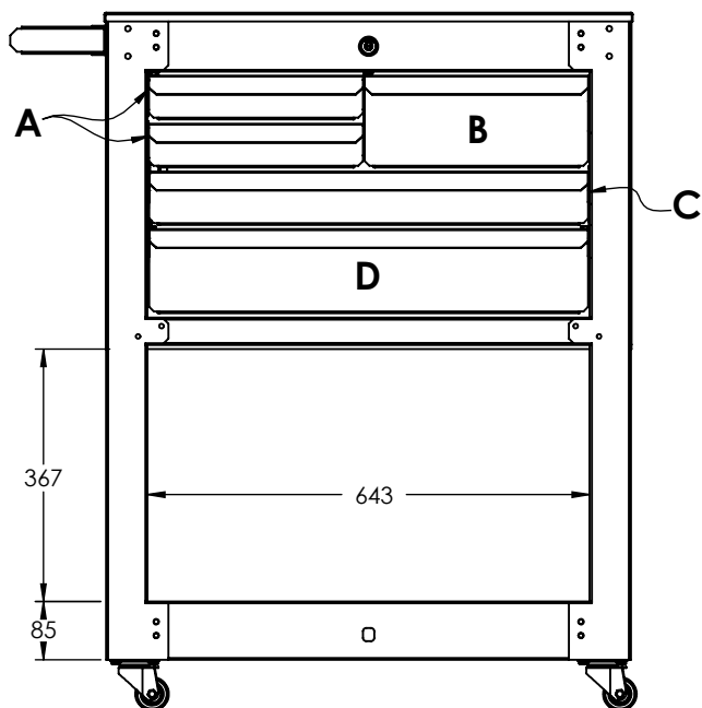
VISTA FRONTAL
