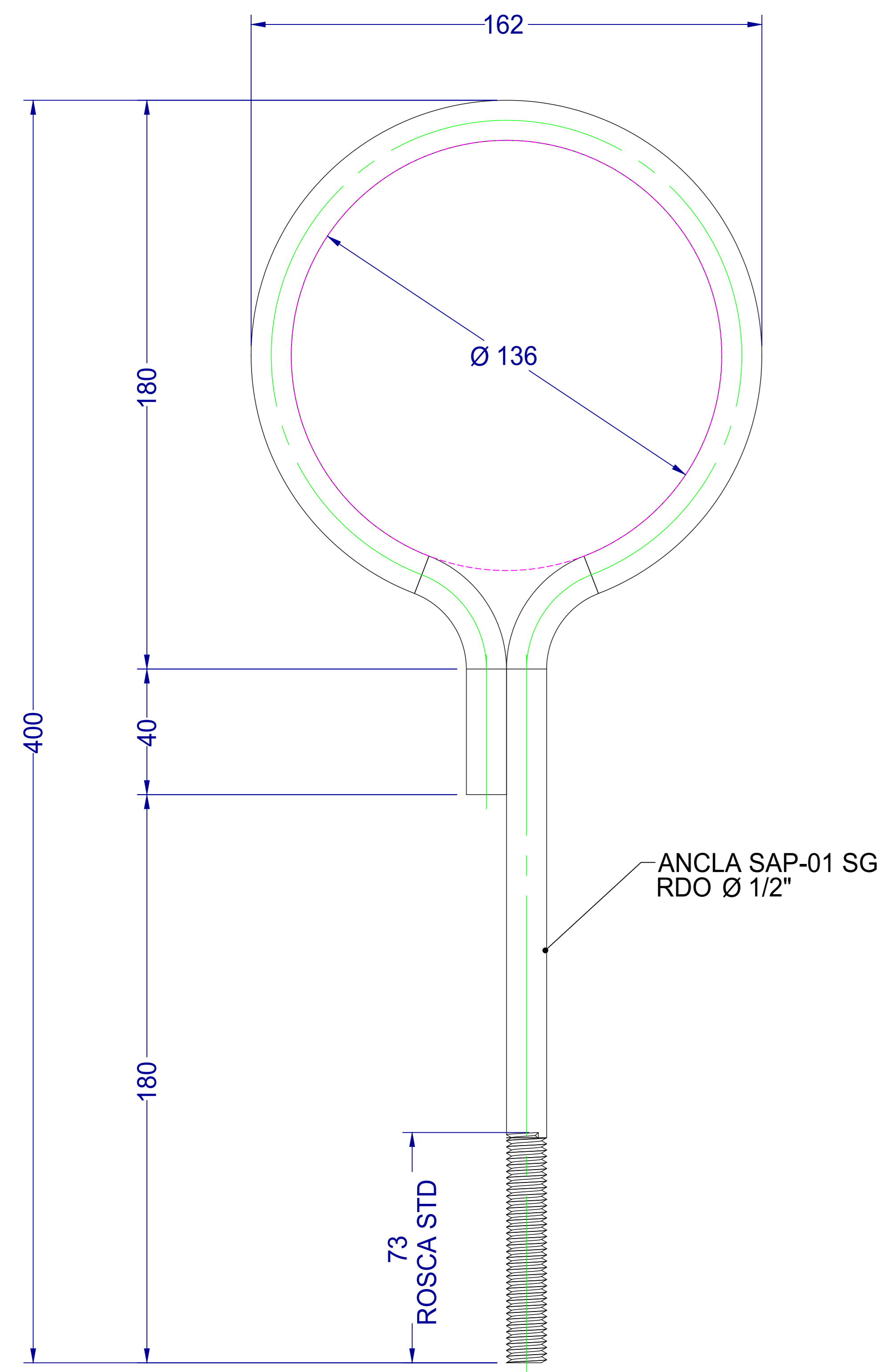
ANCLA SAP-01 SG RDO 1/2"
